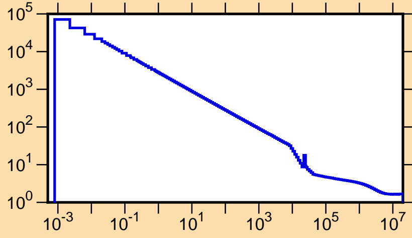
\sigma vs. E for ^{19}\text{Ne}(n,\text{tot.})
