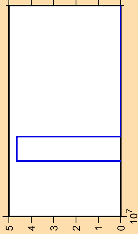
\Delta\sigma/\sigma vs. E for ^{19}\text{Ne}(n,n_1)
