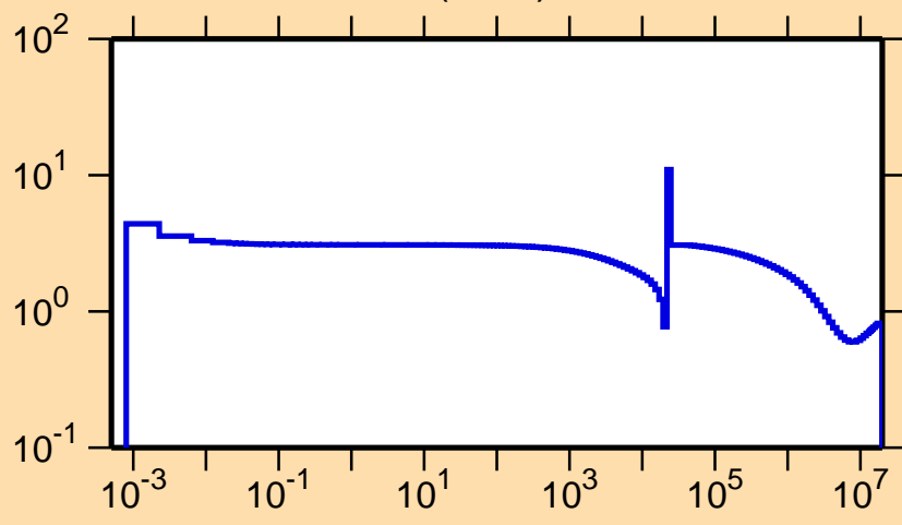
\sigma vs. E for ^{19}\text{Ne}(n,\text{el.})
