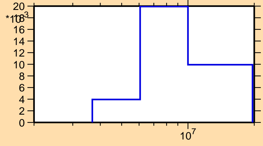
\sigma vs. E for ^{19}\text{Ne}(n,n\text{cont.})
