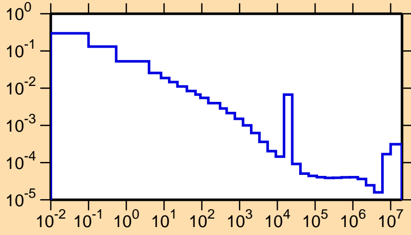
\sigma vs. E for ^{19}\text{Ne}(n,\gamma)
