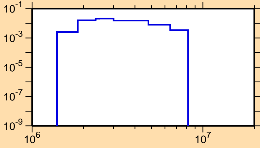
\sigma vs. E for ^{19}\text{Ne}(n,n_4)
