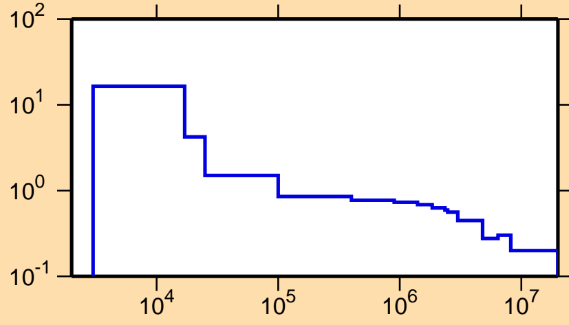
\sigma vs. E for ^{19}\text{Ne}(n,\alpha)
