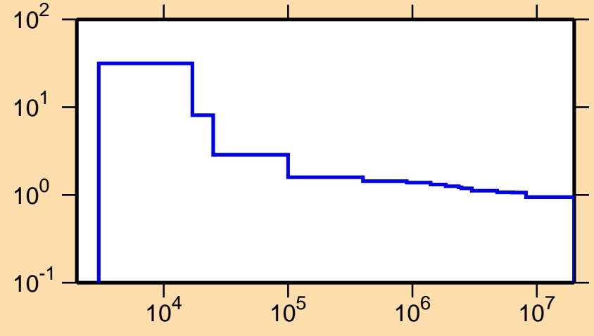
\sigma vs. E for ^{19}\text{Ne}(n,\text{nonel.})
