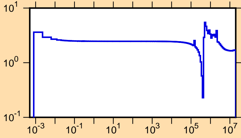
\sigma vs. E for ^{20}\text{Ne}(n,\text{tot.})
