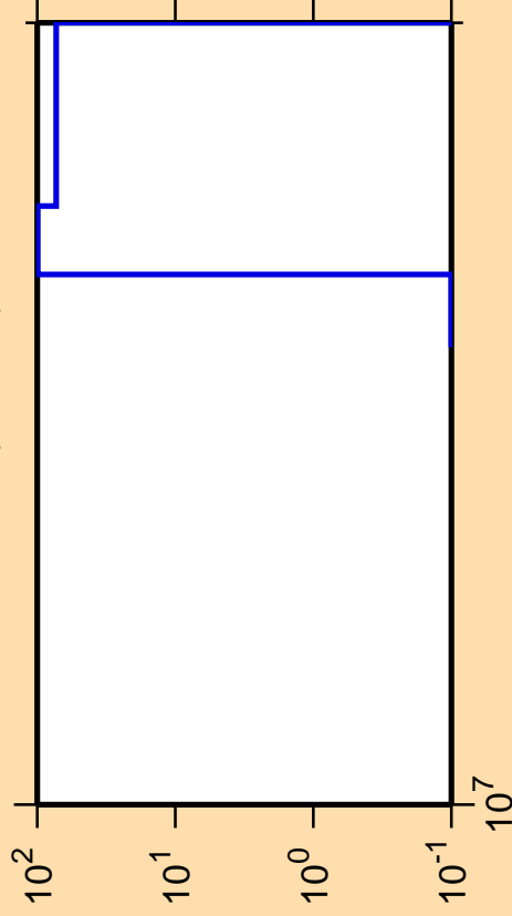
\Delta\sigma/\sigma vs. E for ^{20}\text{Ne}(\text{mt117})
