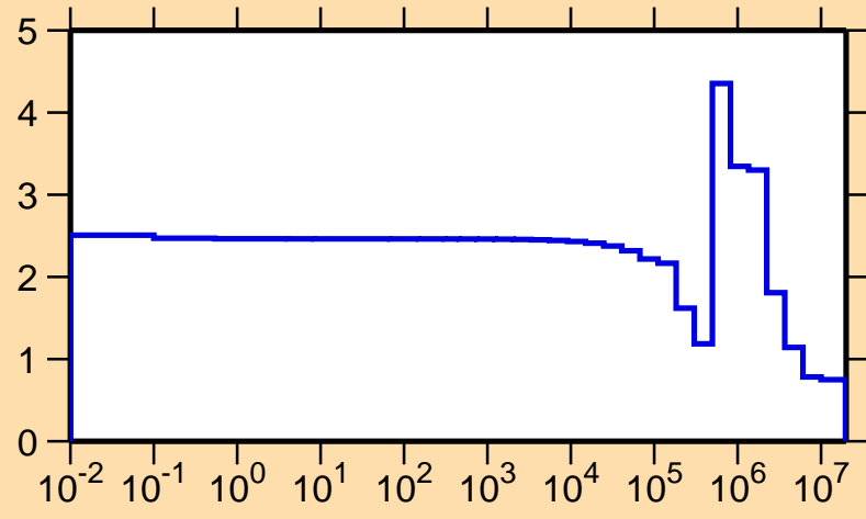
\sigma vs. E for ^{20}\text{Ne}(n,\text{el.})
