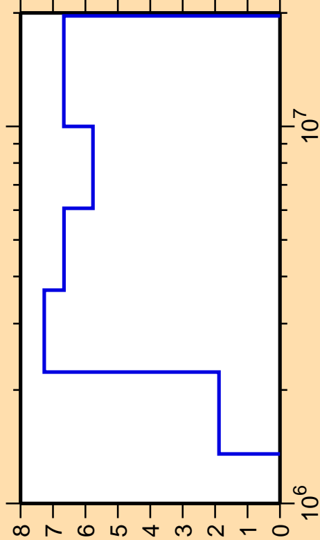
\Delta\sigma/\sigma vs. E for ^{20}\text{Ne}(n,\text{nonel.})
