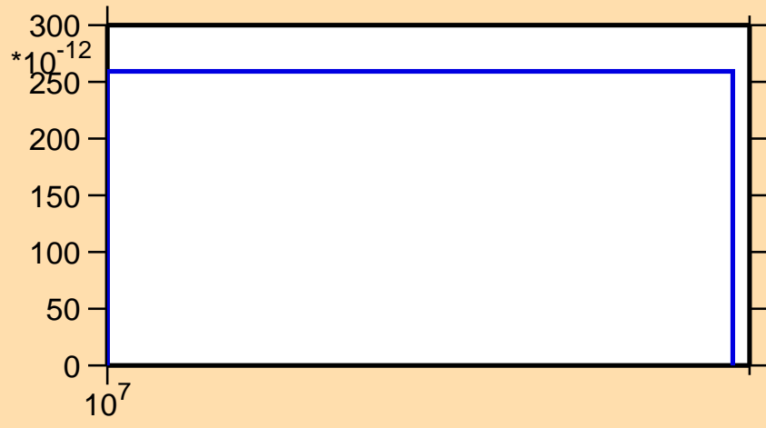
\sigma vs. E for ^{20}\text{Ne} (mt 45)
