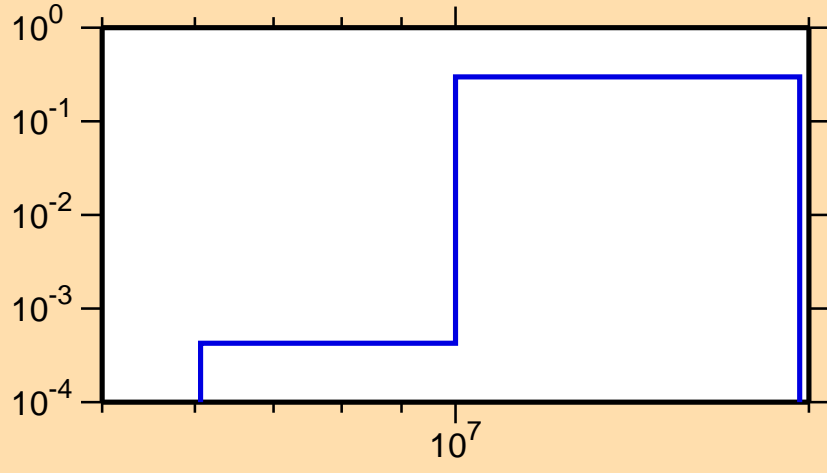
\sigma vs. E for ^{20}\text{Ne}(n,n\alpha)
