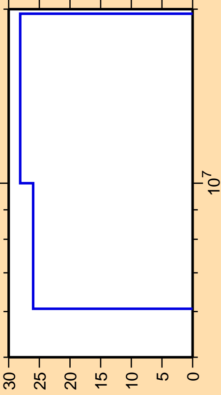
\Delta\sigma/\sigma vs. E for ^{21}\text{Ne}(n,n\text{cont.})
