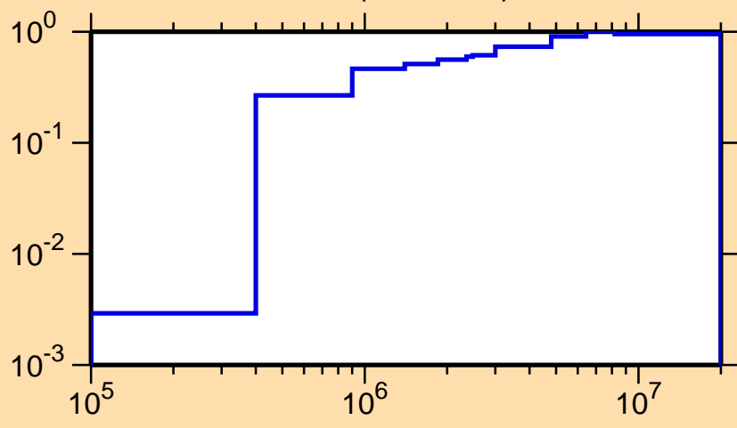
\sigma vs. E for ^{21}\text{Ne}(n,\text{nonel.})
