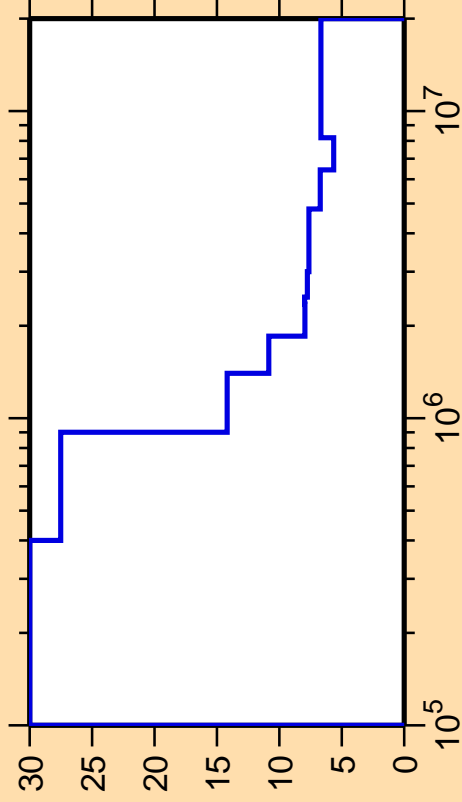
\Delta\sigma/\sigma vs. E for ^{21}\text{Ne}(n,\text{nonel.})
