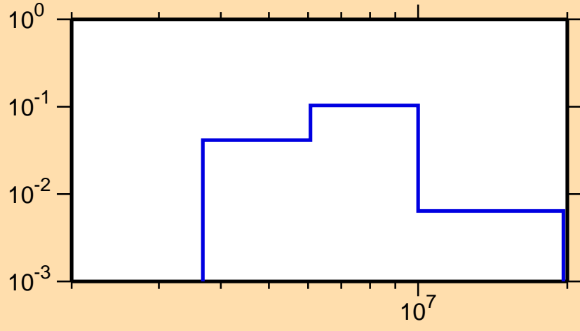
\sigma vs. E for ^{22}\text{Ne}(n,n_3)
