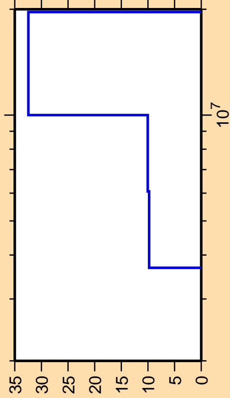
\Delta\sigma/\sigma vs. E for ^{22}\text{Ne}(n,n_3)
