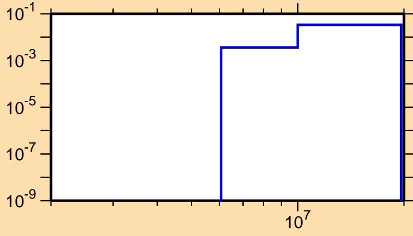
\sigma vs. E for ^{22}\text{Ne}(n,\alpha)
