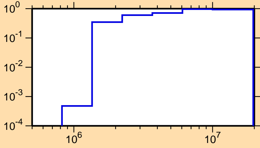
\sigma vs. E for ^{22}\text{Ne}(n,\text{nonel.})
