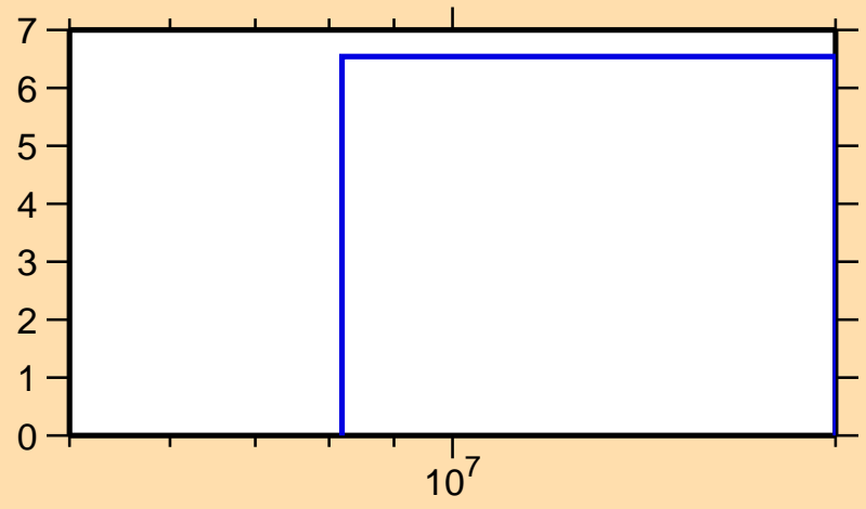
\Delta\sigma/\sigma vs. E for ^{22}\text{Ne}(n,n\text{onel.})
