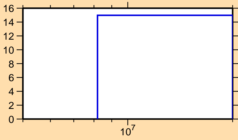
\Delta\sigma/\sigma vs. E for ^{22}\text{Ne}(n,ncont.)
