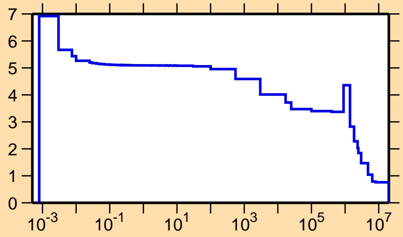
\sigma vs. E for ^{22}\text{Ne}(n,\text{el.})
