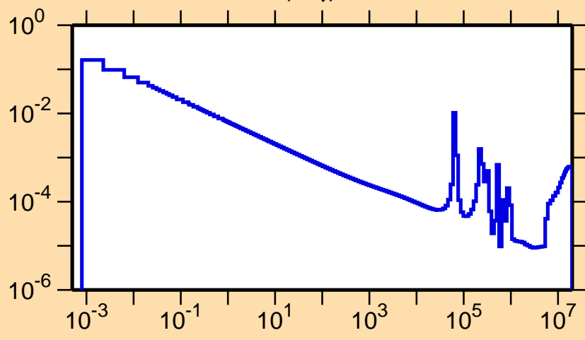
\sigma vs. E for ^{23}\text{Ne}(n,\gamma)
