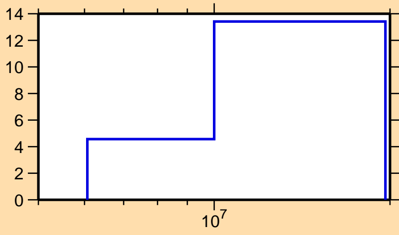
\Delta\sigma/\sigma vs. E for ^{23}\text{Ne}(n,el.)
