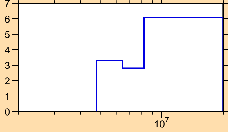
\Delta\sigma/\sigma vs. E for ^{23}\text{Ne}(n,\text{nonel.})
