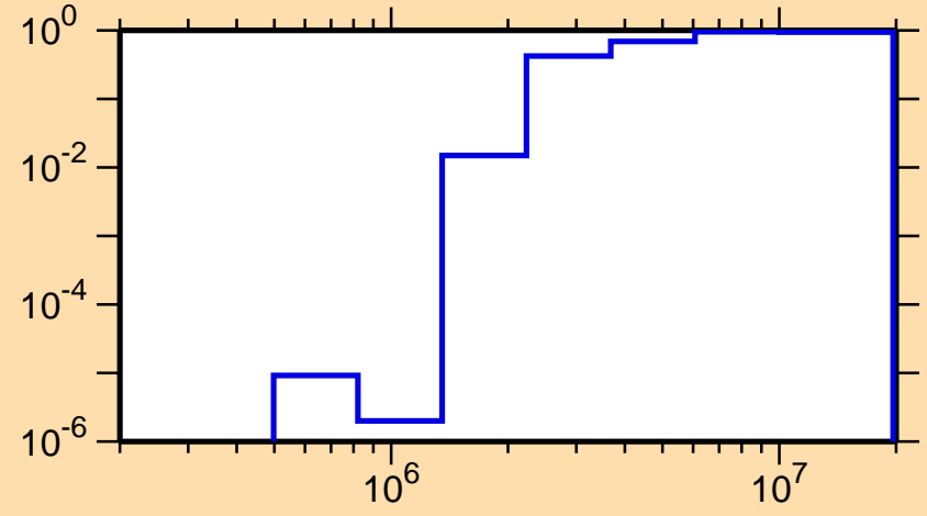
\sigma vs. E for ^{24}\text{Ne}(n,\text{nonel.})
