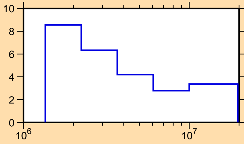
\Delta\sigma/\sigma vs. E for ^{24}\text{Ne}(n,\text{nonel.})
