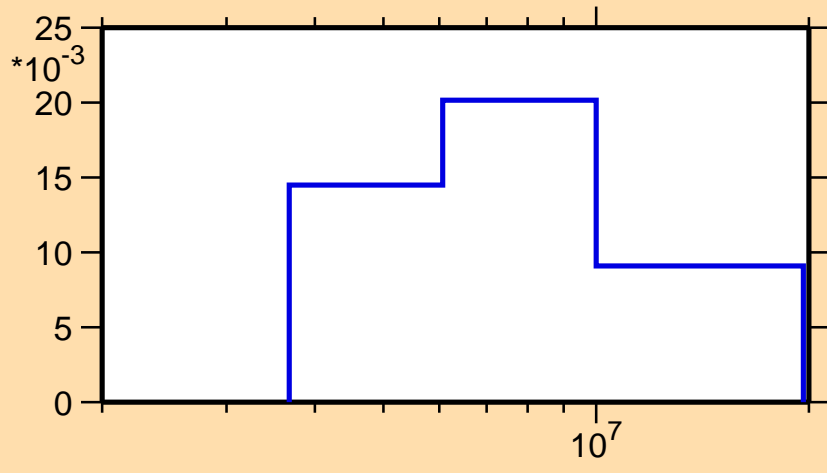
\sigma vs. E for ^{56}\text{Ni}(n,n_2)
