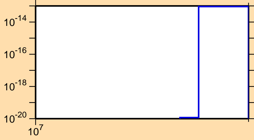
\sigma vs. E for ^{57}\text{Ni} (mt 45)
