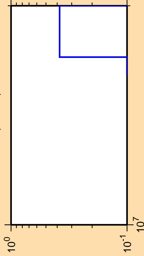
\Delta\sigma/\sigma vs. E for ^{57}\text{Ni} (mt 45)
