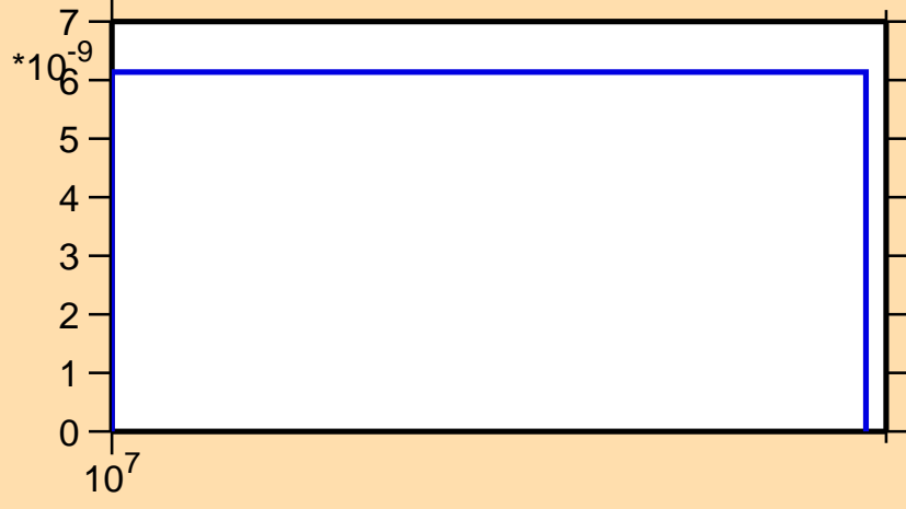
\sigma vs. E for ^{57}\text{Ni}(n,\text{pt})
