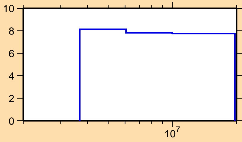
\Delta\sigma/\sigma vs. E for ^{57}\text{Ni}(n,n\text{onel.})
