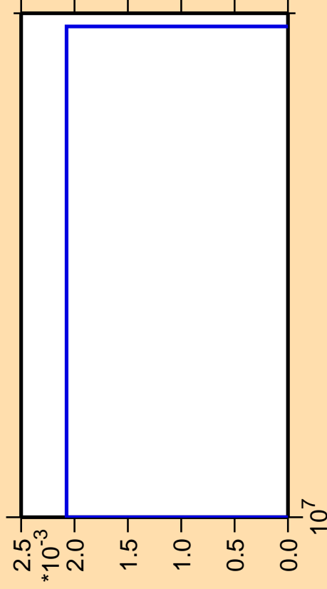
\Delta\sigma/\sigma vs. E for ^{57}\text{Ni} (mt 45)
