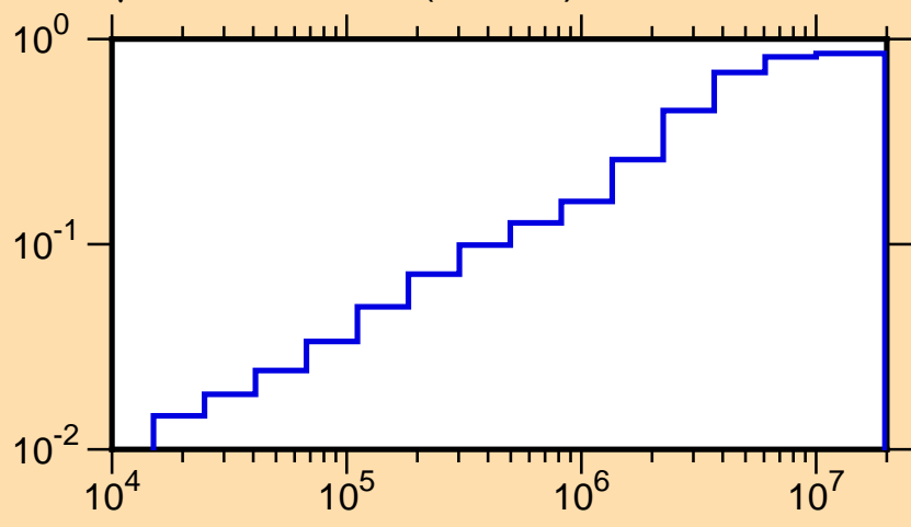
\mu vs. E for ^{58}\text{Ni}(\text{mt251})
