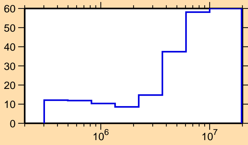
\Delta\sigma/\sigma vs. E for ^{59}\text{Ni}(n,n_1)
