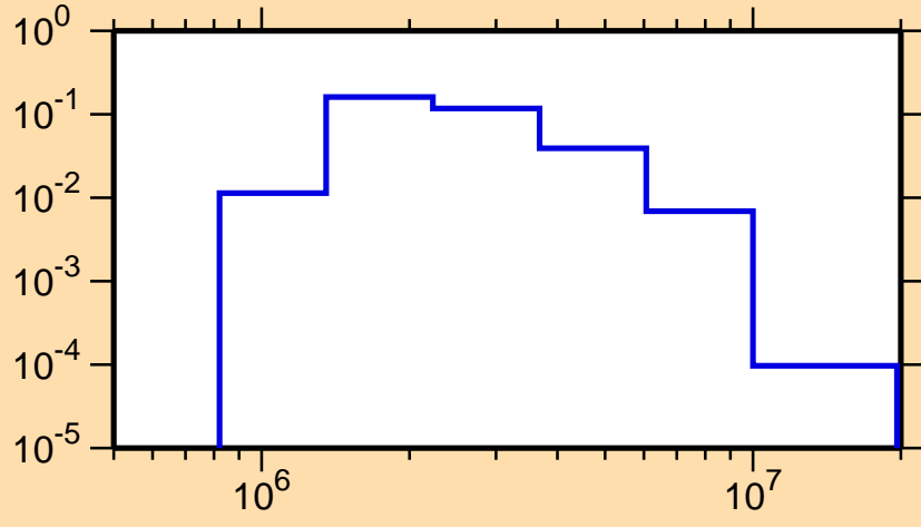
\sigma vs. E for ^{59}\text{Ni}(n,n_4)
