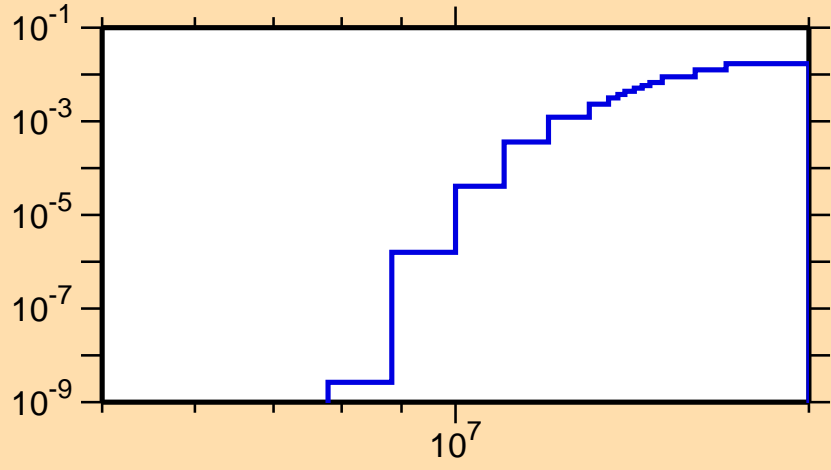
\sigma vs. E for ^{60}\text{Ni}(n,d)
