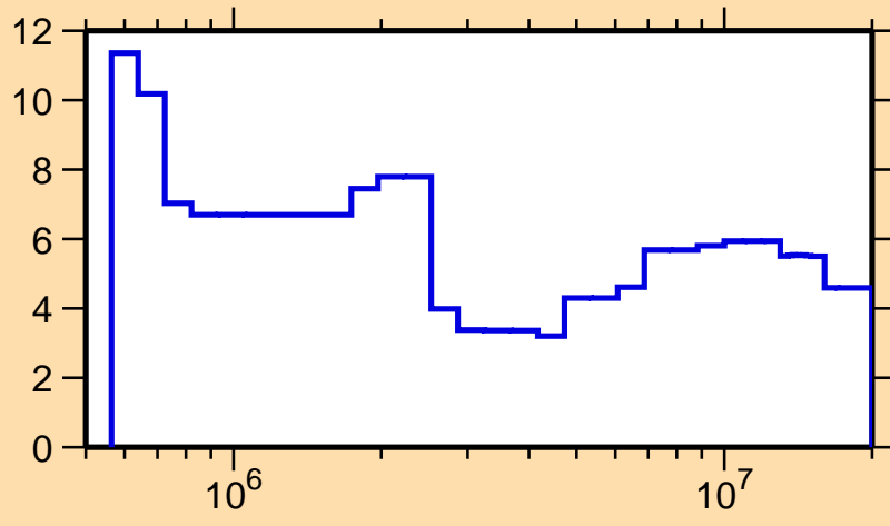
\Delta\sigma/\sigma vs. E for ^{60}\text{Ni}(n,\text{tot.})
