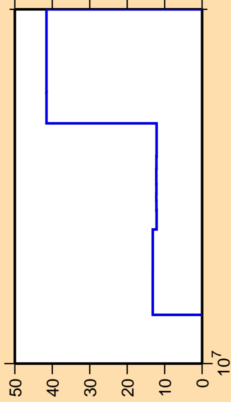
\Delta\sigma/\sigma vs. E for ^{60}\text{Ni}(n,p)
