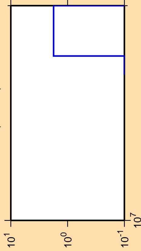
\Delta\sigma/\sigma vs. E for ^{60}\text{Ni}(\text{mt117})
