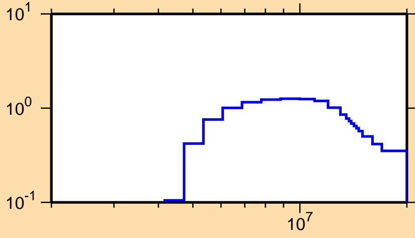
\sigma vs. E for ^{60}\text{Ni}(n,n\text{cont.})
