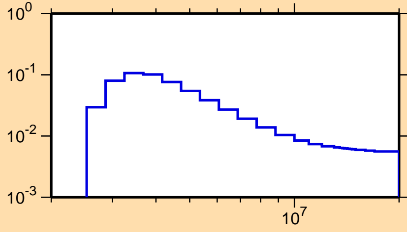
\sigma vs. E for ^{60}\text{Ni}(n,n_4)
