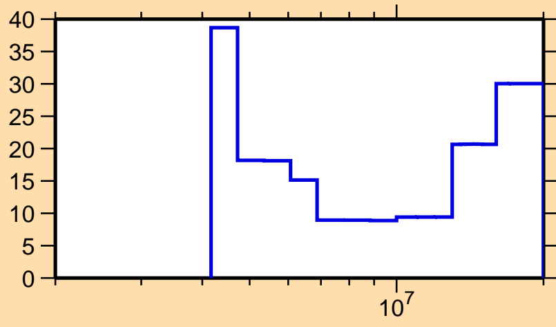
\Delta\sigma/\sigma vs. E for ^{60}\text{Ni}(n,n\text{cont.})
