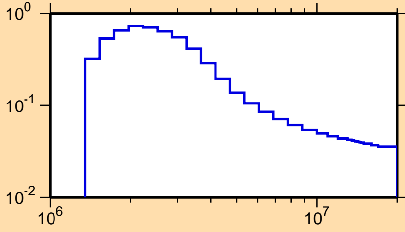
\sigma vs. E for ^{60}\text{Ni}(n,n_1)
