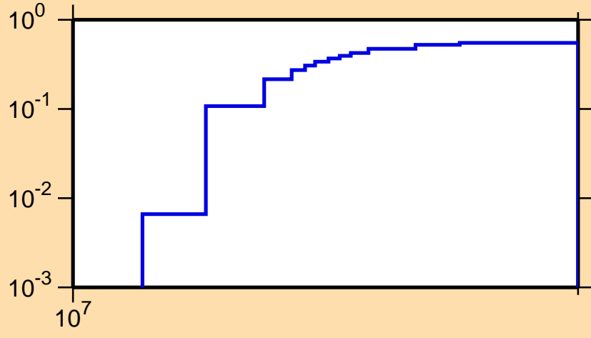
\sigma vs. E for ^{60}\text{Ni}(n,2n)
