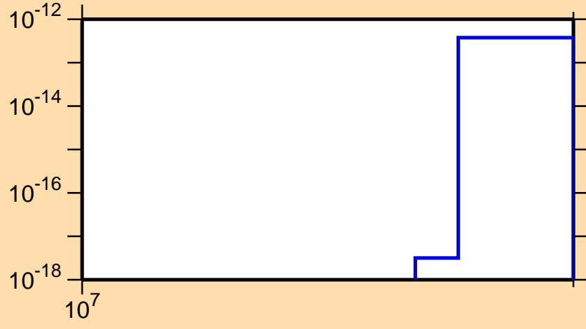
\sigma vs. E for ^{60}\text{Ni}(\text{mt117})
