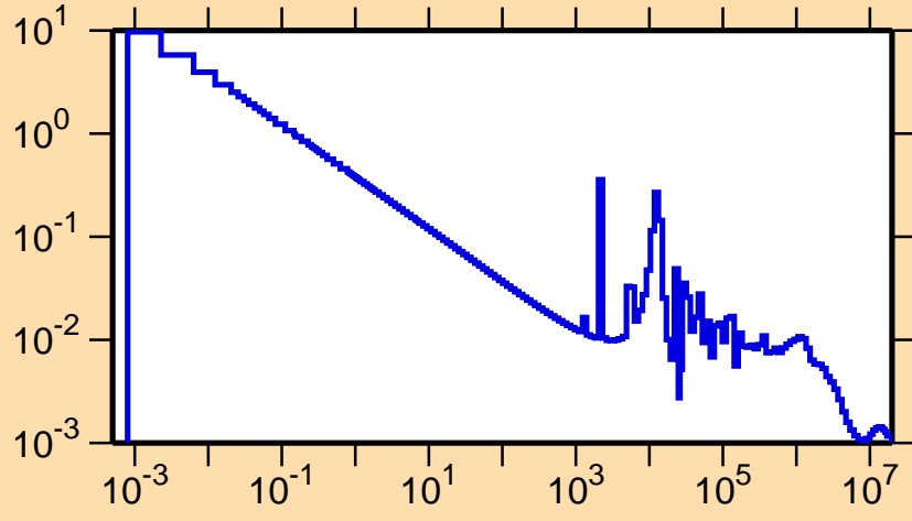
\sigma vs. E for ^{60}\text{Ni}(n,\gamma)
