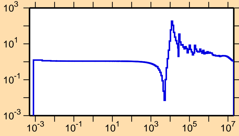
\sigma vs. E for ^{60}\text{Ni}(n,\text{el.})
