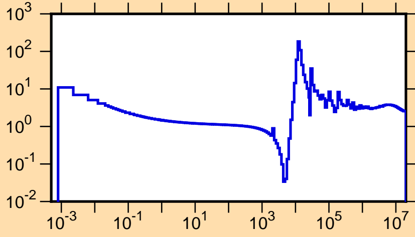
\sigma vs. E for ^{60}\text{Ni}(n,\text{tot.})
