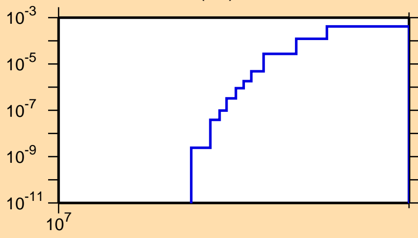
\sigma vs. E for ^{60}\text{Ni}(n,t)
