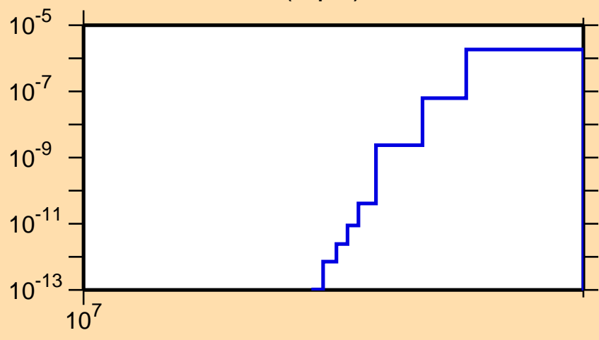
\sigma vs. E for ^{60}\text{Ni}(n,p\alpha)
