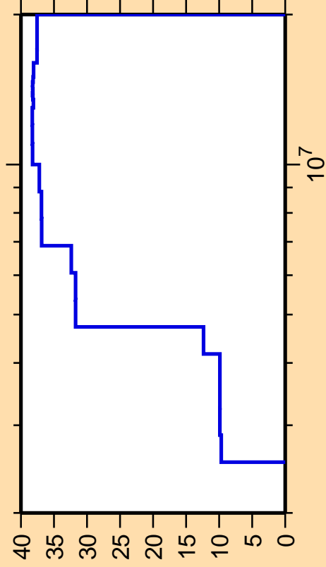
\Delta\sigma/\sigma vs. E for ^{60}\text{Ni}(n,n_4)
