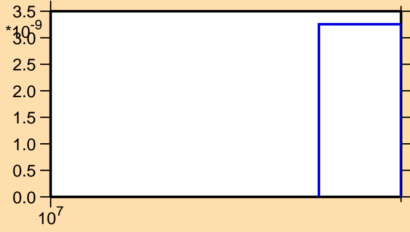
\sigma vs. E for ^{60}\text{Ni}(n,\text{nd})
