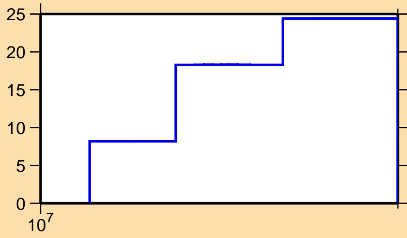
\Delta\sigma/\sigma vs. E for ^{60}\text{Ni}(n,\text{inel.})
