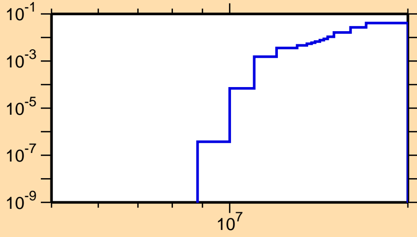
\sigma vs. E for ^{60}\text{Ni}(n,n\alpha)
