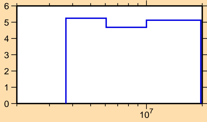
\Delta\sigma/\sigma vs. E for ^{60}\text{Ni}(n,n\text{nonel.})
