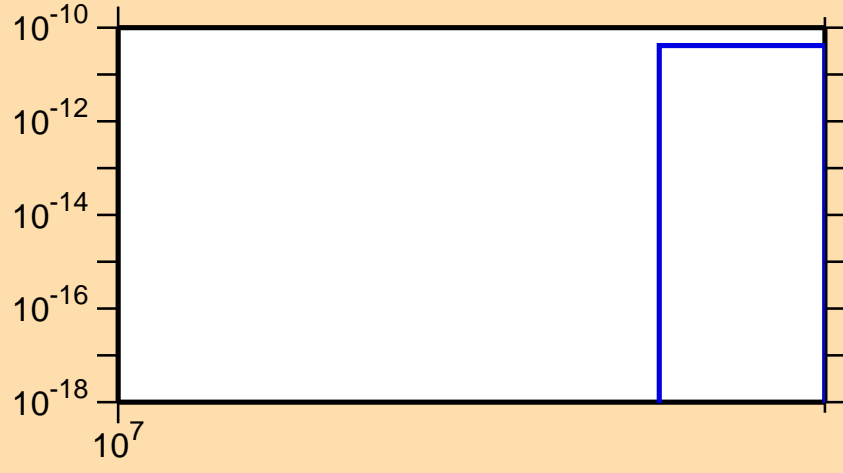
\sigma vs. E for ^{61}\text{Ni}(n,\text{pt})
