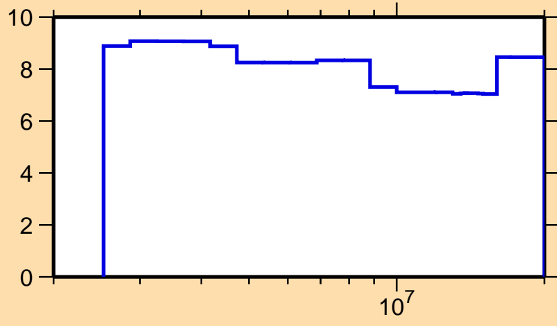
\Delta\sigma/\sigma vs. E for ^{61}\text{Ni}(n,n\text{onel.})
