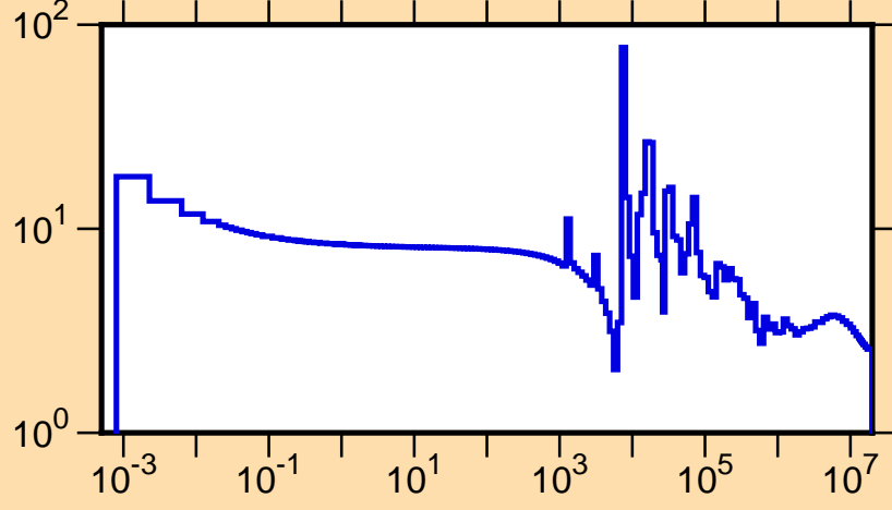
\sigma vs. E for ^{61}\text{Ni}(n,\text{tot.})
