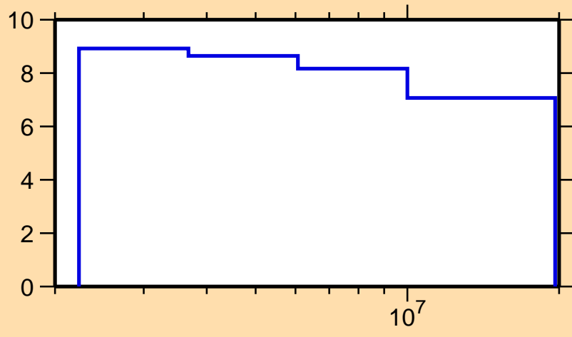
\Delta\sigma/\sigma vs. E for ^{61}\text{Ni}(n,n\text{nonel.})
