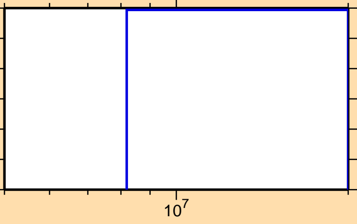
\sigma vs. E for ^{61}\text{Ni}(n,\text{He3})
