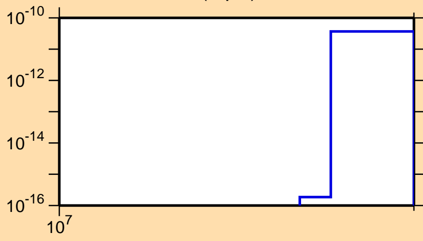
\sigma vs. E for ^{62}\text{Ni}(n,p\alpha)
