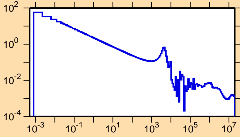
\sigma vs. E for ^{62}\text{Ni}(n,\gamma)
