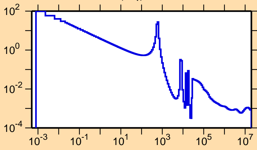
\sigma vs. E for ^{63}\text{Ni}(n,\gamma)
