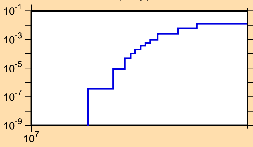
\sigma vs. E for ^{63}\text{Ni}(n,np)
