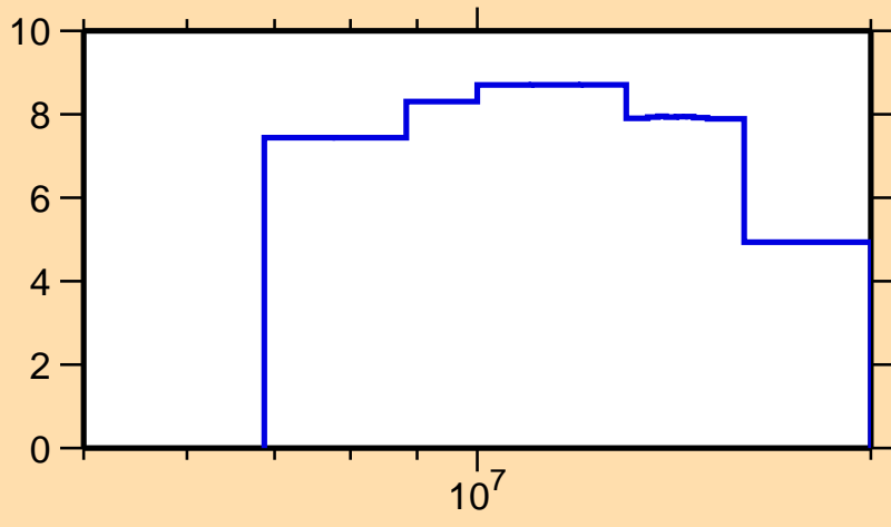
\Delta\sigma/\sigma vs. E for ^{63}\text{Ni}(n,\text{tot.})
