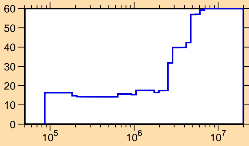
\Delta\sigma/\sigma vs. E for ^{63}\text{Ni}(n,n_1)
