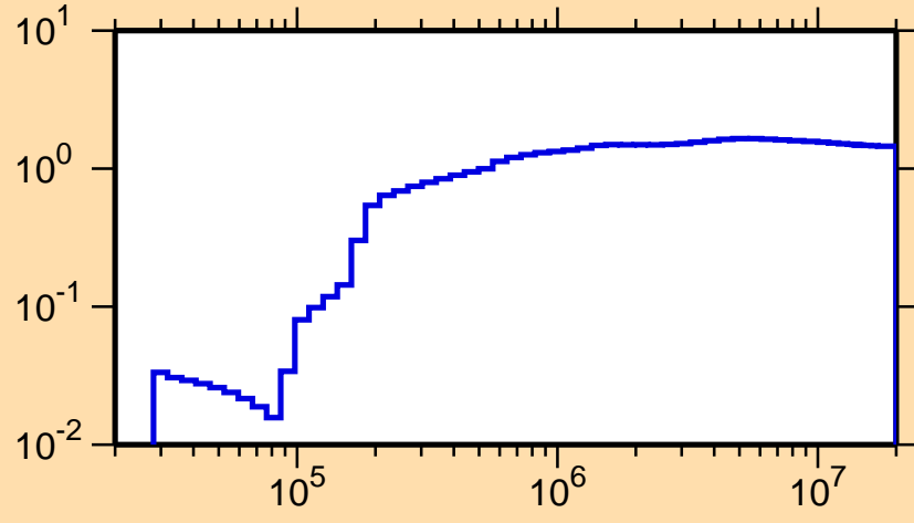
\sigma vs. E for ^{63}\text{Ni}(n,\text{nonel.})
