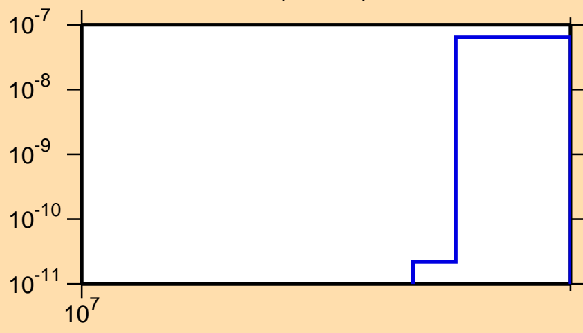
\sigma vs. E for ^{63}\text{Ni}(n,2n\alpha)
