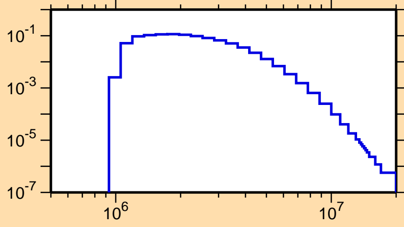
\sigma vs. E for ^{63}\text{Ni}(n,n_4)
