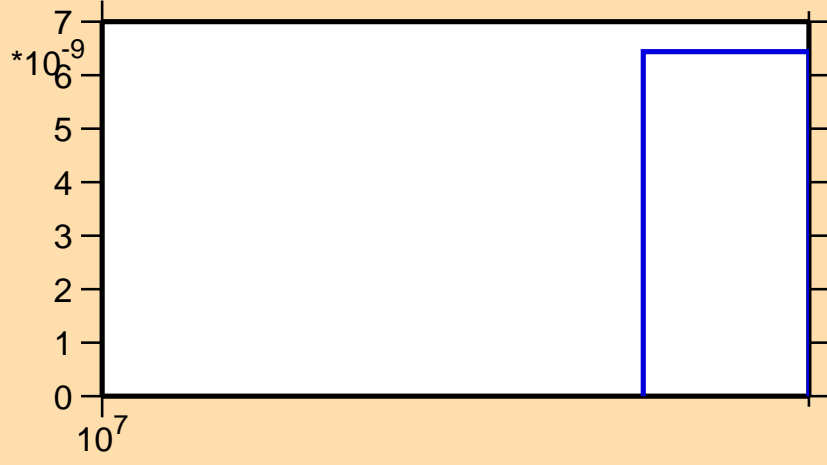
\sigma vs. E for ^{63}\text{Ni}(n,2np)
