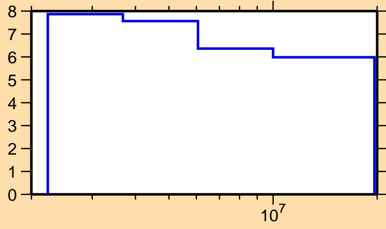
\Delta\sigma/\sigma vs. E for ^{63}\text{Ni}(n,n\text{onel.})
