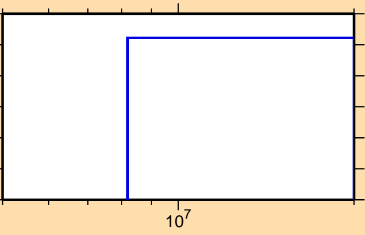
\sigma vs. E for ^{63}\text{Ni}(n,2n\alpha)
