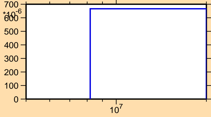
\sigma vs. E for ^{63}\text{Ni}(n,d)
