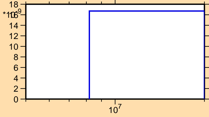
\sigma vs. E for ^{63}\text{Ni}(n,\text{nd})
