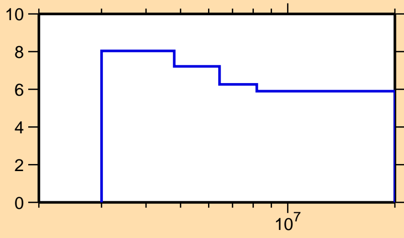
\Delta\sigma/\sigma vs. E for ^{63}\text{Ni}(n,n\text{onel.})
