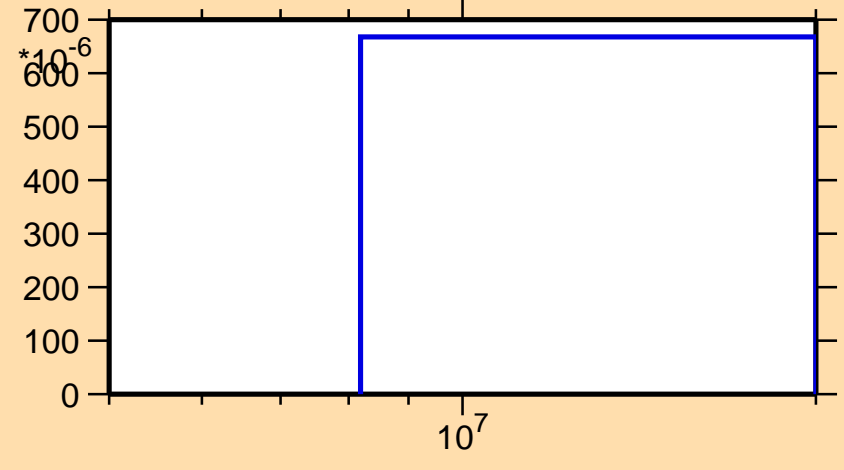
\sigma vs. E for ^{63}\text{Ni}(n,n\alpha)
