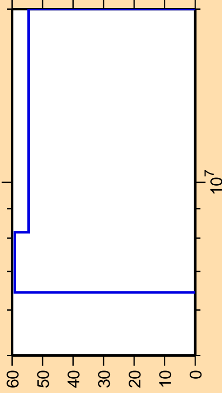
\Delta\sigma/\sigma vs. E for ^{63}\text{Ni}(n,\alpha)
