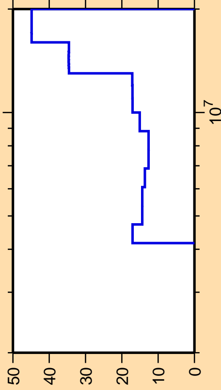
\Delta\sigma/\sigma vs. E for ^{64}\text{Ni}(n,\text{ncont.})
