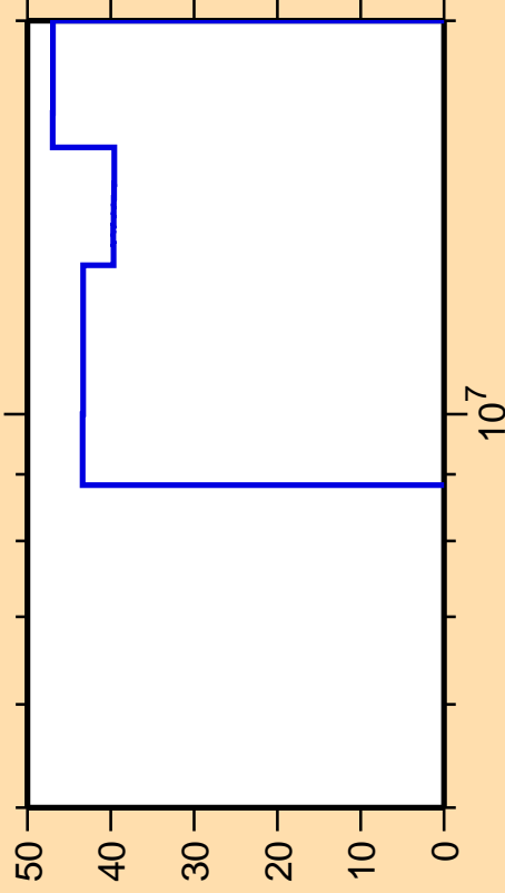
\Delta\sigma/\sigma vs. E for ^{64}\text{Ni}(n,p)
