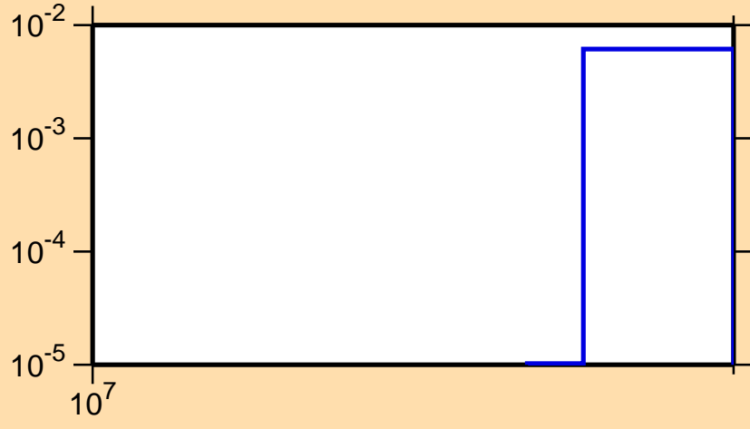
\sigma vs. E for ^{64}\text{Ni}(n,3n)
