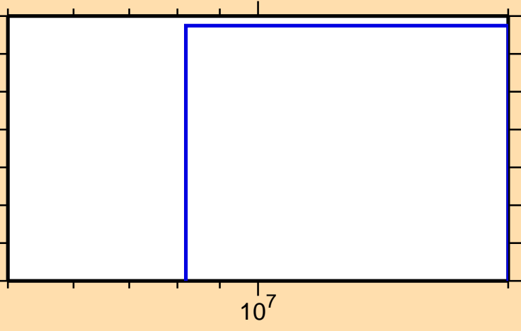
\sigma vs. E for ^{64}\text{Ni}(n,d)
