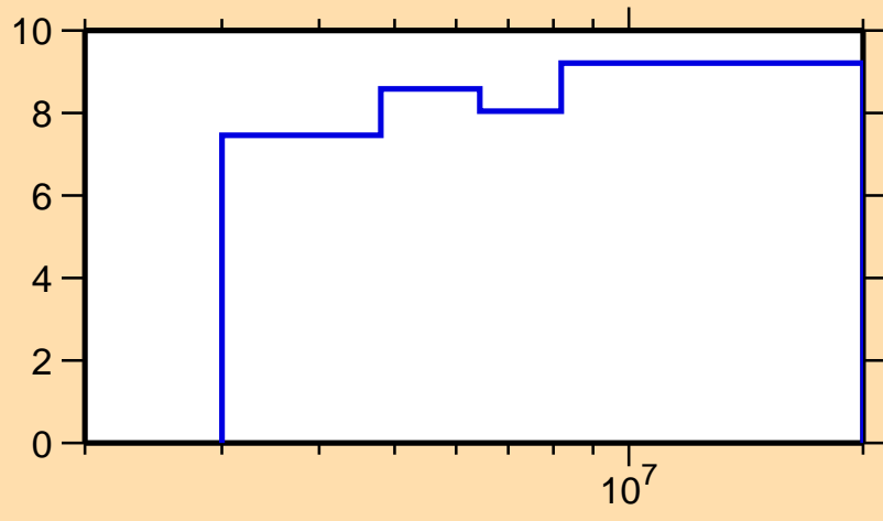
\Delta\sigma/\sigma vs. E for ^{65}\text{Ni}(n,n\text{nonel.})
