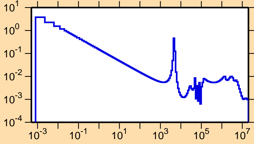
\sigma vs. E for ^{66}\text{Ni}(n,\gamma)
