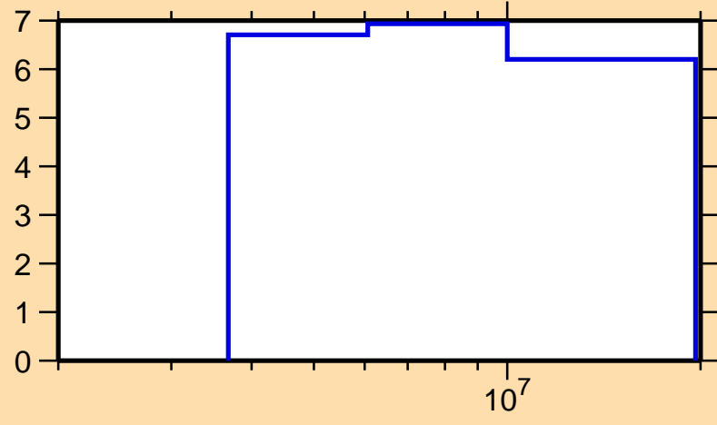
\Delta\sigma/\sigma vs. E for ^{66}\text{Ni}(n,n\text{nonel.})
