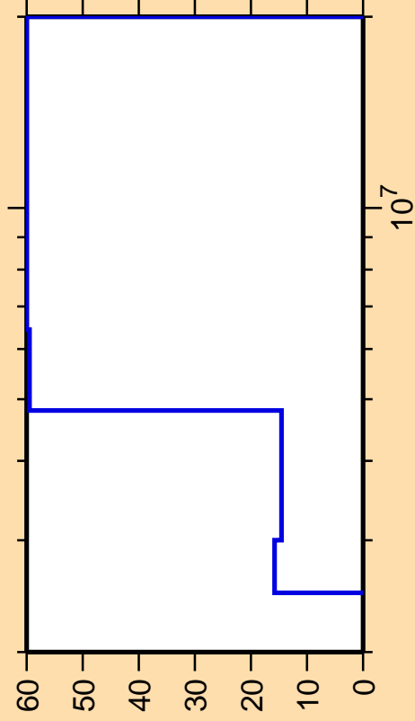
\Delta\sigma/\sigma vs. E for ^{66}\text{Ni}(n,n_3)
