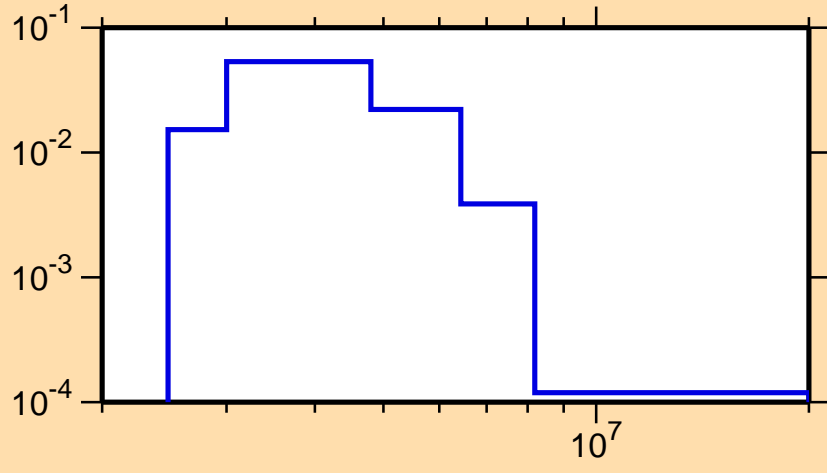
\sigma vs. E for ^{66}\text{Ni}(n,n_3)
