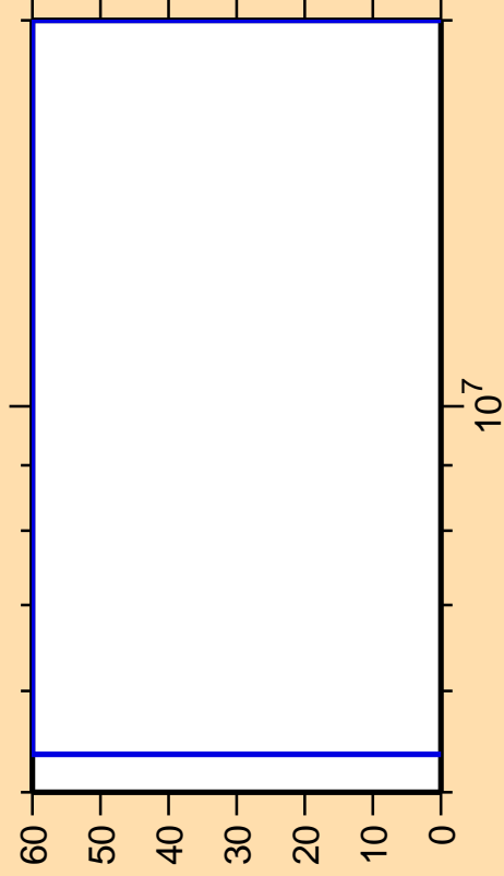
\Delta\sigma/\sigma vs. E for ^{67}\text{Ni}(n,\gamma)
