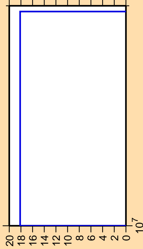
\Delta\sigma/\sigma vs. E for ^{67}\text{Ni}(n,nd)
