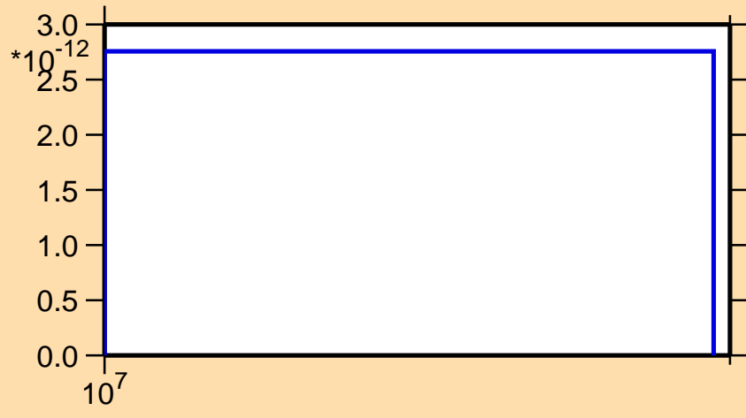
\sigma vs. E for ^{67}\text{Ni}(n,nd)
