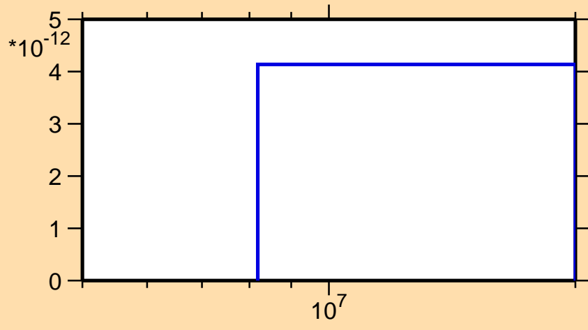
\sigma vs. E for ^{67}\text{Ni}(n,\text{nd})
