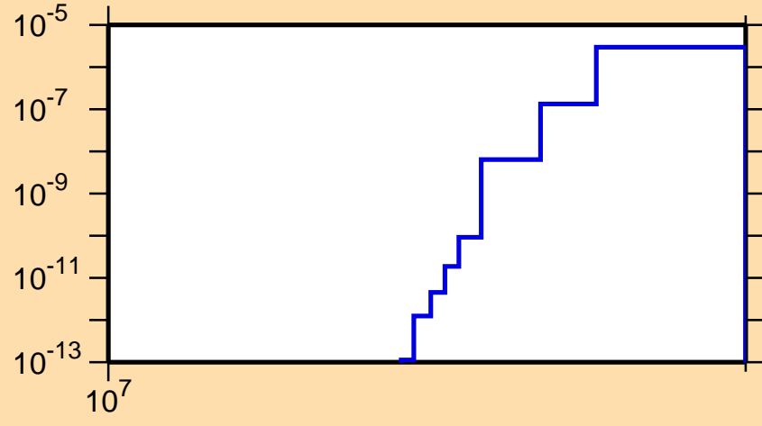
\sigma vs. E for ^{68}\text{Ni}(n,n\alpha)
