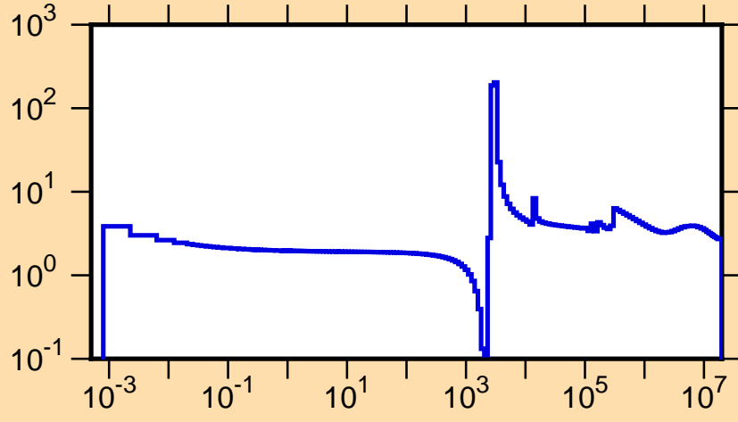
\sigma vs. E for ^{68}\text{Ni}(n,\text{tot.})
