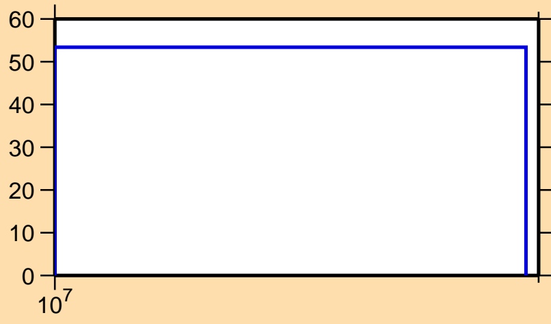
\Delta\sigma/\sigma vs. E for ^{68}\text{Ni}(n,\gamma)
