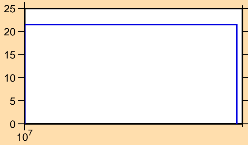
\Delta\sigma/\sigma vs. E for ^{68}\text{Ni}(n,2n)
