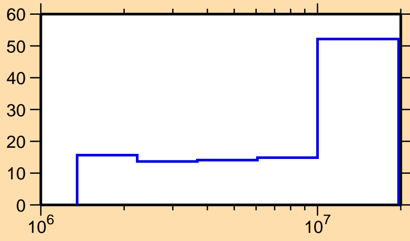
\Delta\sigma/\sigma vs. E for ^{68}\text{Ni}(n,\text{inel.})
