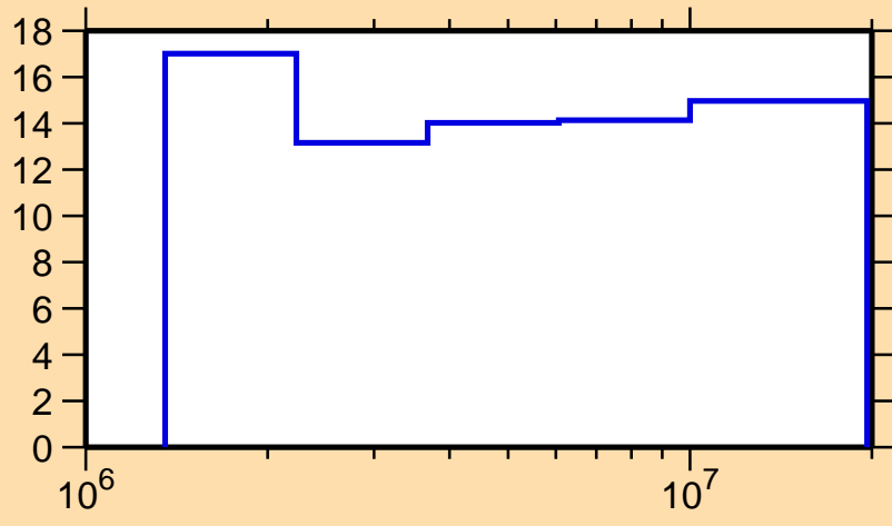
\Delta\sigma/\sigma vs. E for ^{68}\text{Ni}(n,\text{nonel.})
