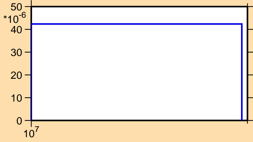
\sigma vs. E for ^{68}\text{Ni}(n,p)
