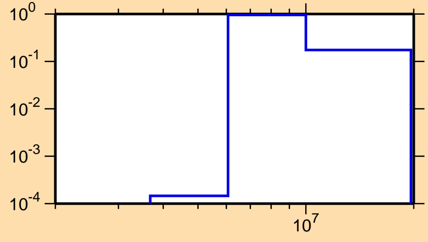
\sigma vs. E for ^{68}\text{Ni}(n,n\text{cont.})
