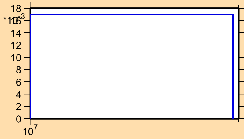
\sigma vs. E for ^{68}\text{Ni}(n,3n)
