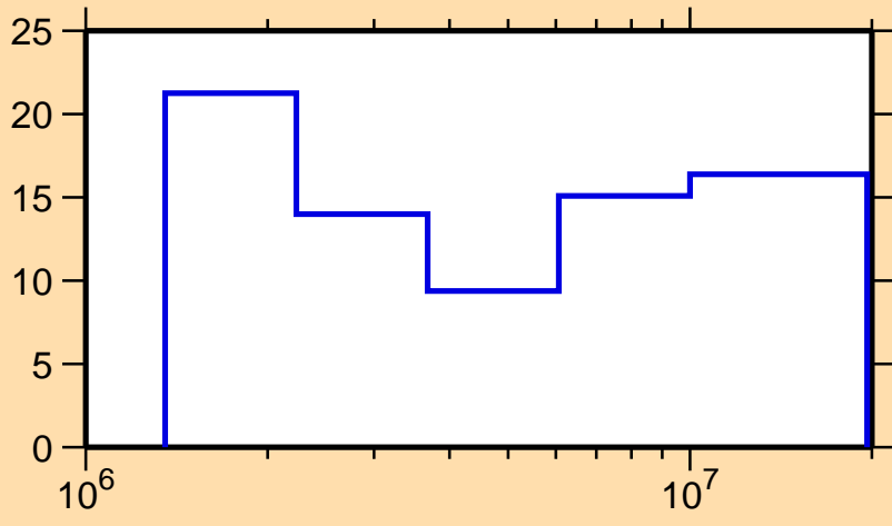
\Delta\sigma/\sigma vs. E for ^{68}\text{Ni}(n,\text{tot.})
