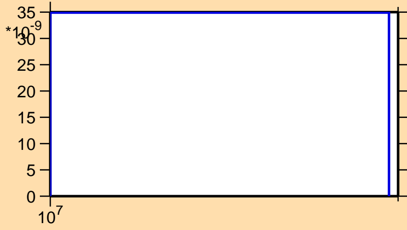
\sigma vs. E for ^{68}\text{Ni}(n,n\alpha)
