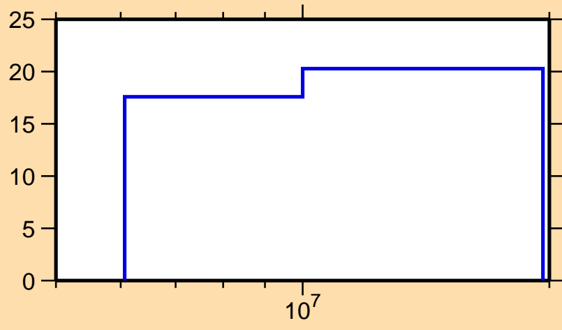
\Delta\sigma/\sigma vs. E for ^{68}\text{Ni}(n,\text{el.})
