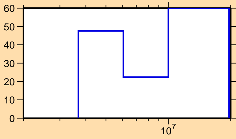
\Delta\sigma/\sigma vs. E for ^{68}\text{Ni}(n,n\text{cont.})
