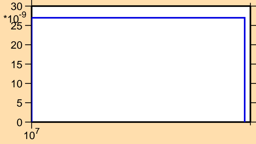
\sigma vs. E for ^{68}\text{Ni}(n,t)
