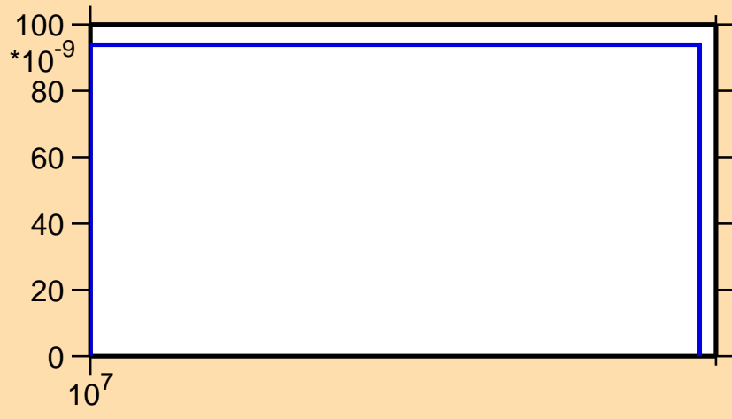
\sigma vs. E for ^{68}\text{Ni}(n,np)
