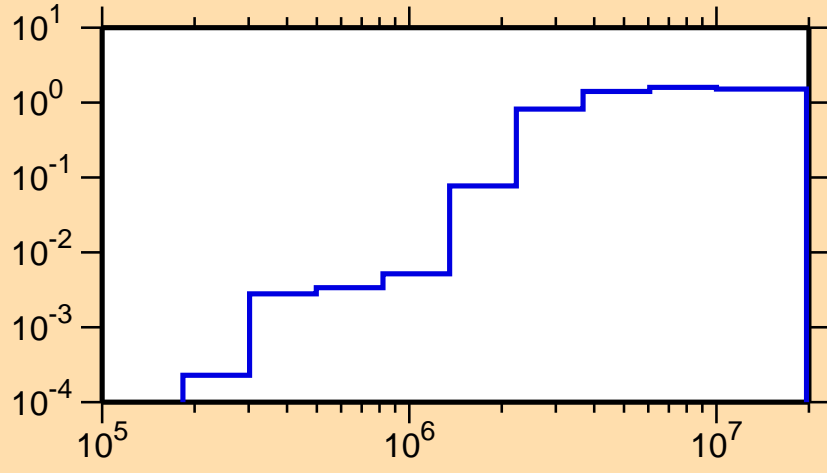
\sigma vs. E for ^{68}\text{Ni}(n,\text{nonel.})
