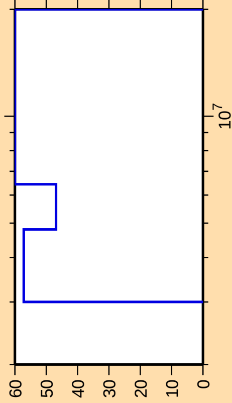
\Delta\sigma/\sigma vs. E for ^{69}\text{Ni}(n,\text{ncont.})
