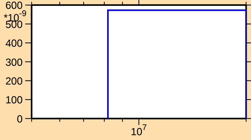
\sigma vs. E for ^{69}\text{Ni}(n,t)
