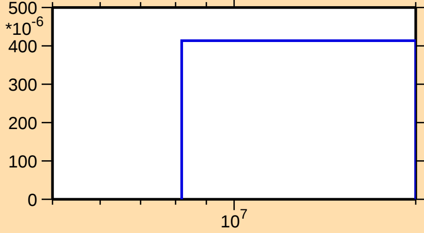
\sigma vs. E for ^{69}\text{Ni}(n,p)
