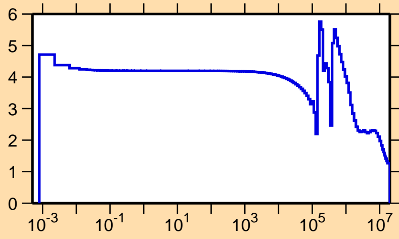
\sigma vs. E for ^{70}\text{Ni}(n,\text{el.})
