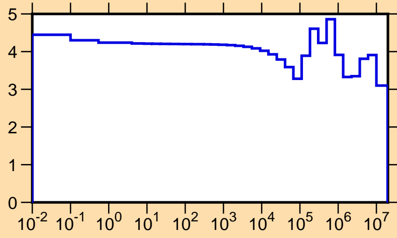
\sigma vs. E for ^{70}\text{Ni}(n,\text{tot.})
