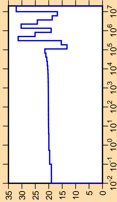
\Delta\sigma/\sigma vs. E for ^{70}\text{Ni}(n,\text{tot.})
