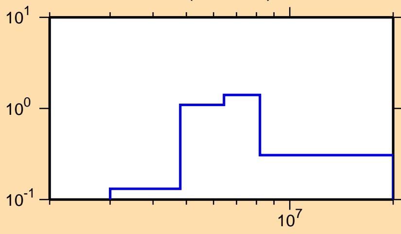
\sigma vs. E for ^{70}\text{Ni}(n,n\text{cont.})
