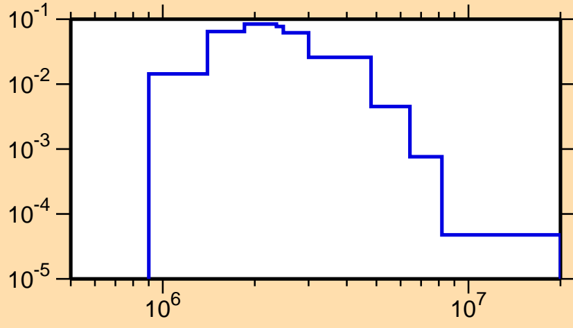
\sigma vs. E for ^{71}\text{Ni}(n,n_4)
