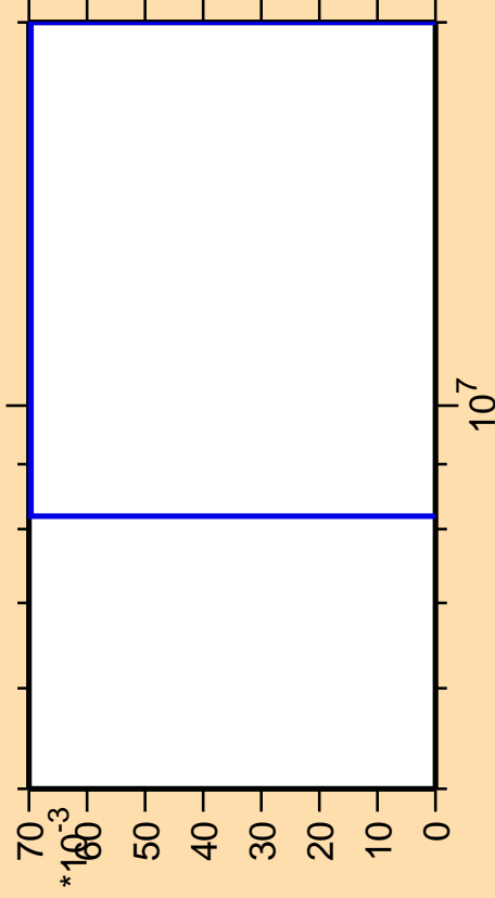
\Delta\sigma/\sigma vs. E for ^{71}\text{Ni}(n,\text{nd})
