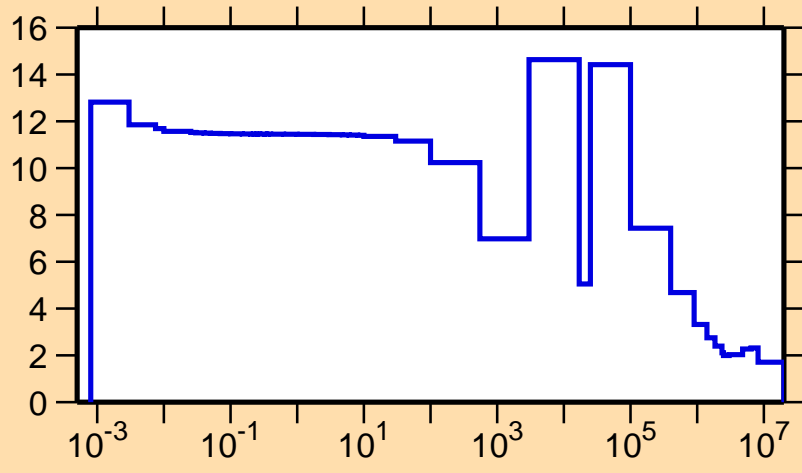
\sigma vs. E for ^{71}\text{Ni}(n,\text{el.})
