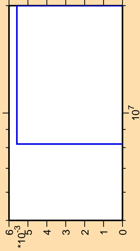
\Delta\sigma/\sigma vs. E for ^{71}\text{Ni}(n,nt)
