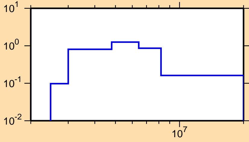
\sigma vs. E for ^{71}\text{Ni}(n,n\text{cont.})
