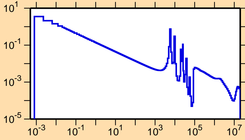
\sigma vs. E for ^{71}\text{Ni}(n,\gamma)
