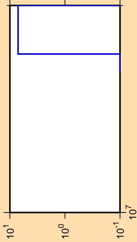
\Delta\sigma/\sigma vs. E for ^{71}\text{Ni}(n,2n\alpha)
