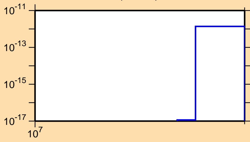
\sigma vs. E for ^{71}\text{Ni}(n,2n\alpha)
