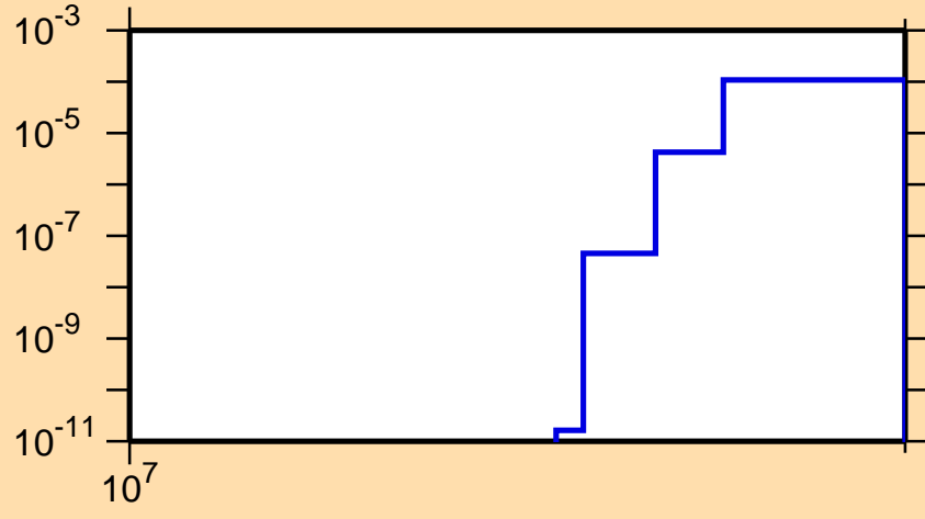
\sigma vs. E for ^{71}\text{Ni}(n,d)
