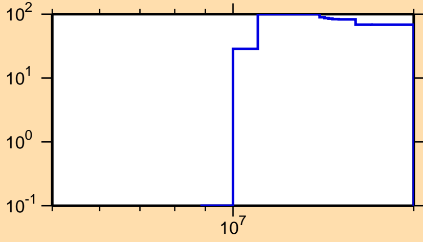
\Delta\sigma/\sigma vs. E for ^{71}\text{Ni}(n,p)
