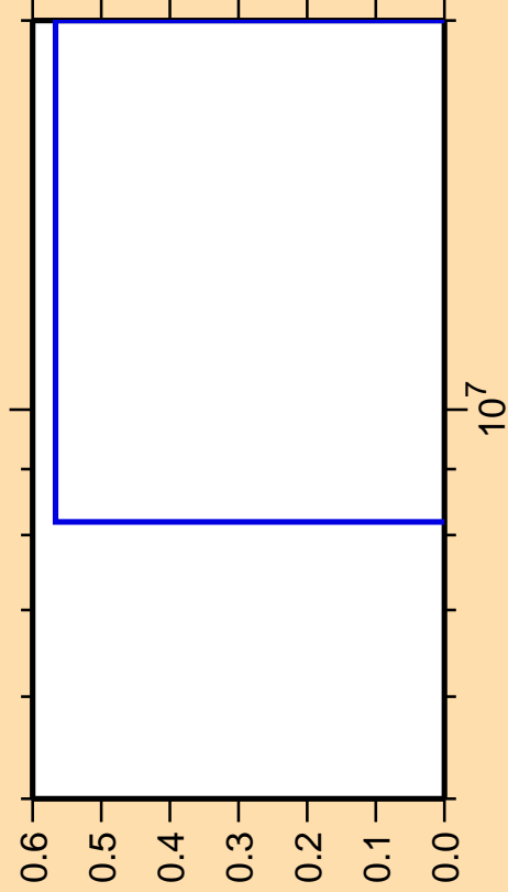
\Delta\sigma/\sigma vs. E for ^{71}\text{Ni}(n,\text{nt})
