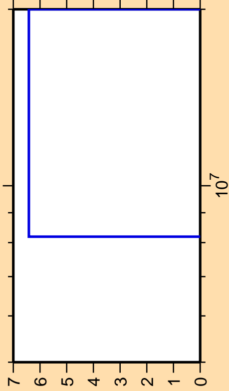
\Delta\sigma/\sigma vs. E for ^{71}\text{Ni}(n,\text{nd})
