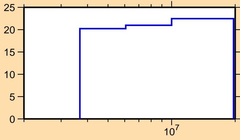
\Delta\sigma/\sigma vs. E for ^{72}\text{Ni}(n,n\text{onel.})
