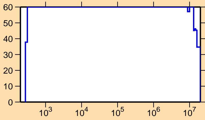
\Delta\sigma/\sigma vs. E for ^{251}\text{No}(n,\gamma)
