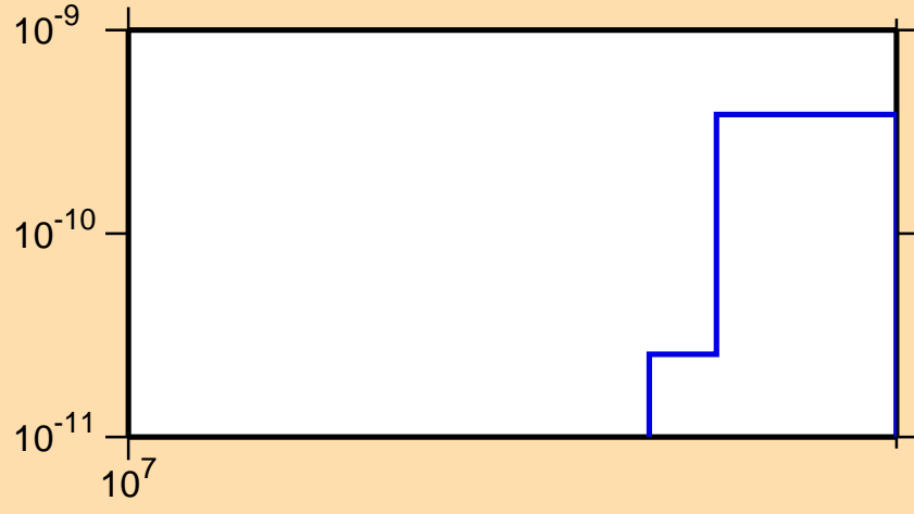
\sigma vs. E for ^{251}\text{No}(\text{mt } 34)
