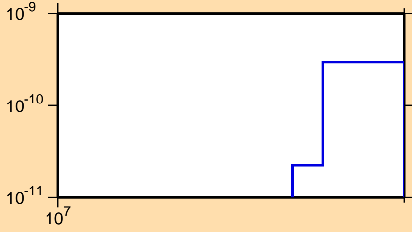
\sigma vs. E for ^{251}\text{No}(n,\text{pt})
