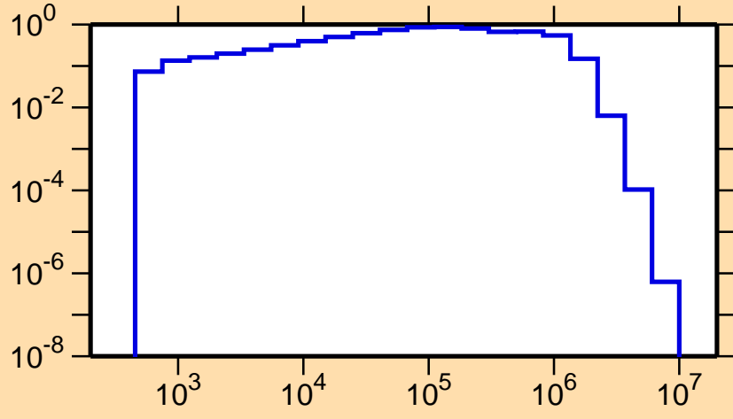
\sigma vs. E for ^{251}\text{No}(n,n_1)
