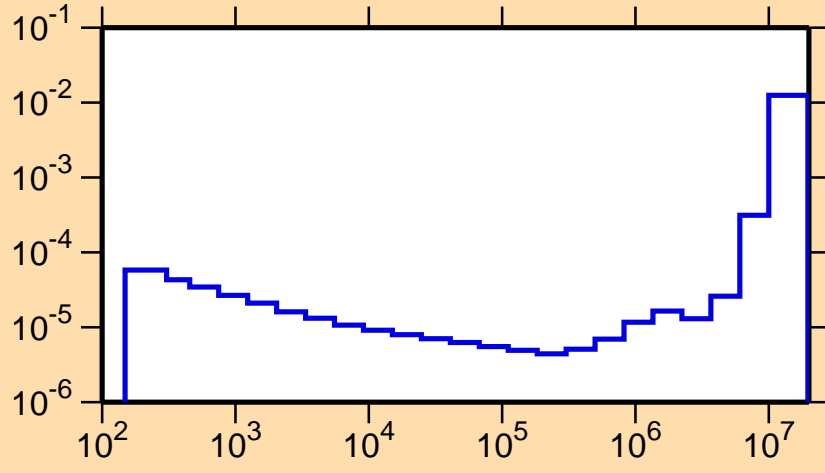
\sigma vs. E for ^{251}\text{No}(n,p)
