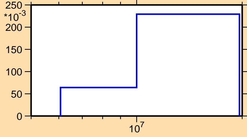
\sigma vs. E for ^{251}\text{No}(n,2n)
