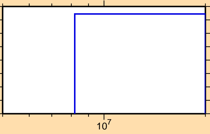
\sigma vs. E for ^{251}\text{No}(n,\text{pd})
