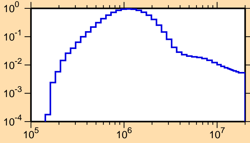
\sigma vs. E for ^{252}\text{No}(n,n_2)
