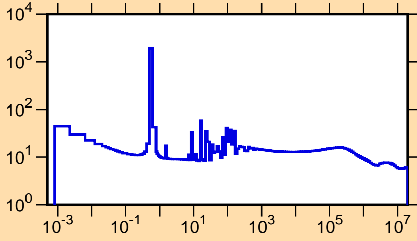
\sigma vs. E for ^{252}\text{No}(n,\text{tot.})
