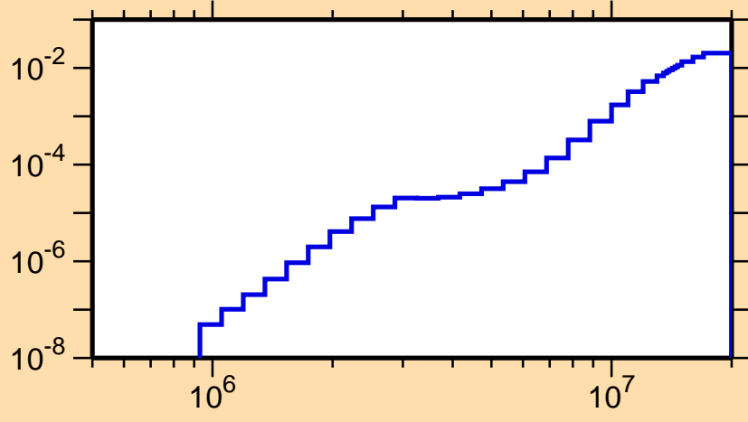
\sigma vs. E for ^{252}\text{No}(n,p)
