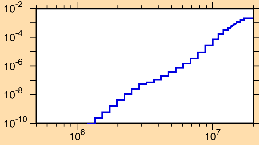
\sigma vs. E for ^{252}\text{No}(n,p\alpha)
